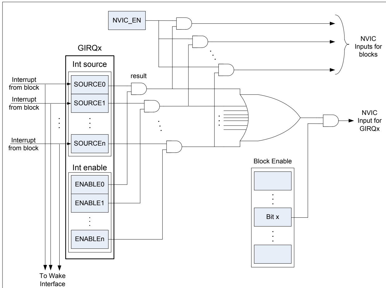
FIGURE 9-2: INTERRUPT STRUCTURE
