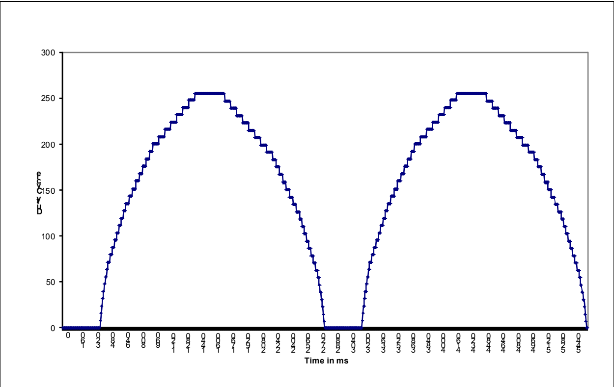
FIGURE 21-6: NON-LINEAR BRIGHTNESS CURVE EXAMPLE
