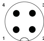
Pin assignment of M12 male connector, 4-pos., A-coded, view
