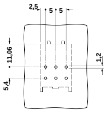
Drilling diagram VC-AMLV 6
