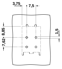
Drilling diagram VC-AMLV 2
