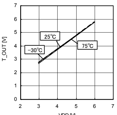
Fig.20 T_OUT Output High Voltage (source 1mA)
