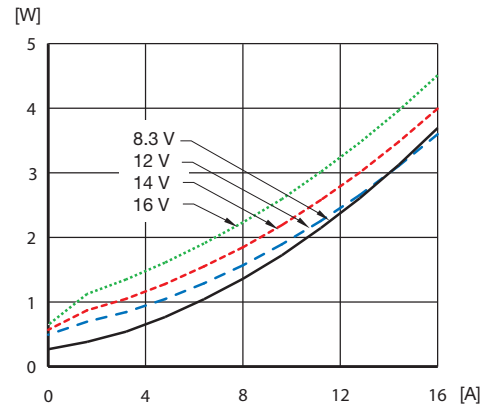
Dissipated power vs. load current and input voltage at T_{\text{ref}} = +25^\circ\text{C}
