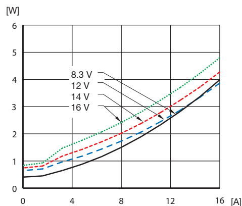
Dissipated power vs. load current and input voltage at T_{ref} = +25\text{ °C}
