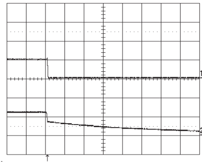
Turn-off at I_O = 16\text{ A} resistive load at T_{\text{ref}} = +25^\circ\text{C} , V_{\text{in}} = 12\text{ V} . Turn-off enabled by disconnecting V_{\text{in}} . Top trace: output voltage (1 V/div.). Bottom trace: input voltage (10 V/div.). Time scale: 2 ms/div.
