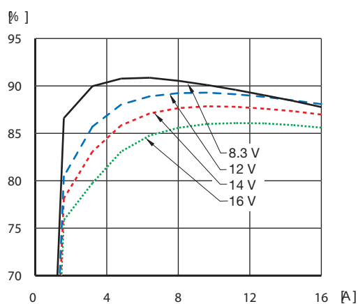
Efficiency vs. load current and input voltage at T_{ref} = +25\text{ °C}
