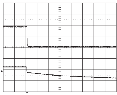
Turn-off at I_O = 16\text{ A} resistive load at T_{ref} = +25\text{ °C} , V_{in} = 12\text{ V} . Turn-off enabled by disconnecting V_{in} . Top trace: output voltage (1 V/div.). Bottom trace: input voltage (10 V/div.). Time scale: 2 ms/div.
