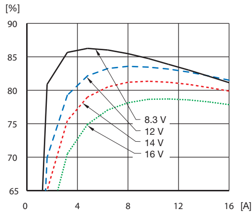
Efficiency vs. load current and input voltage at T_{\text{ref}} = +25^\circ\text{C}
