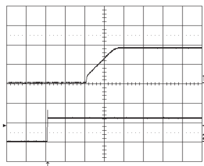
Start-up at I_O = 16\text{ A} resistive load at T_{ref} = +25\text{ °C} , V_{in} = 12\text{ V} . Start enabled by connecting V_{in} . Top trace: output voltage (1 V/div.). Bottom trace: input voltage (10 V/div.). Time scale: 2 ms/div.
