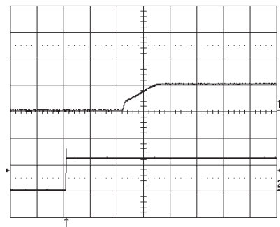
Start-up at I_O = 16\text{ A} resistive load at T_{\text{ref}} = +25^\circ\text{C} , V_{\text{in}} = 12\text{ V} . Start enabled by connecting V_{\text{in}} . Top trace: output voltage (1 V/div.). Bottom trace: input voltage (10 V/div.). Time scale: 2 ms/div.
