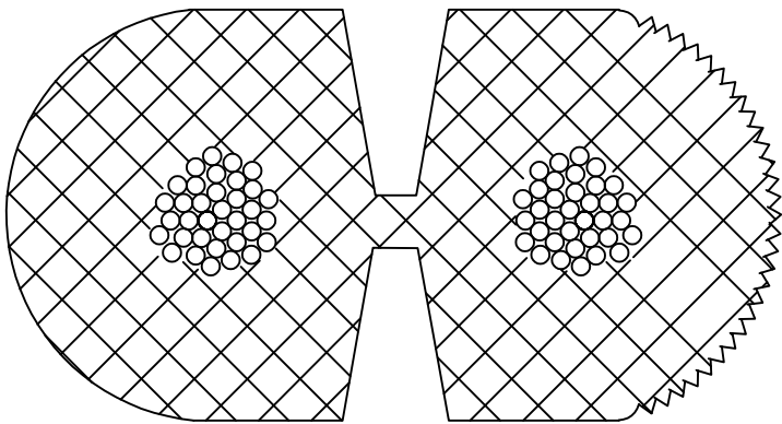
CROSS SECTION OF SPT-2 CABLE
