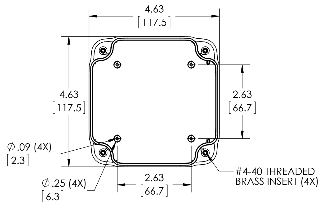
INSIDE VIEW OF COVER
