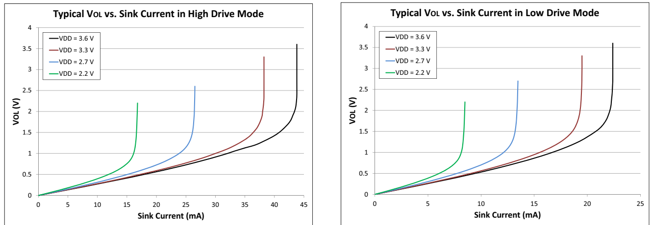
Figure 1.6. Typical V_{OL} vs. Sink Current
