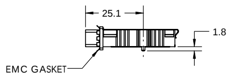
EMC GASKET
