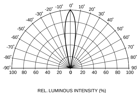
Fig. 5 Radiation Diagram
