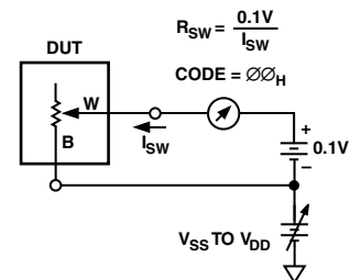
Figure 17. Incremental ON Resistance Test Circuit
