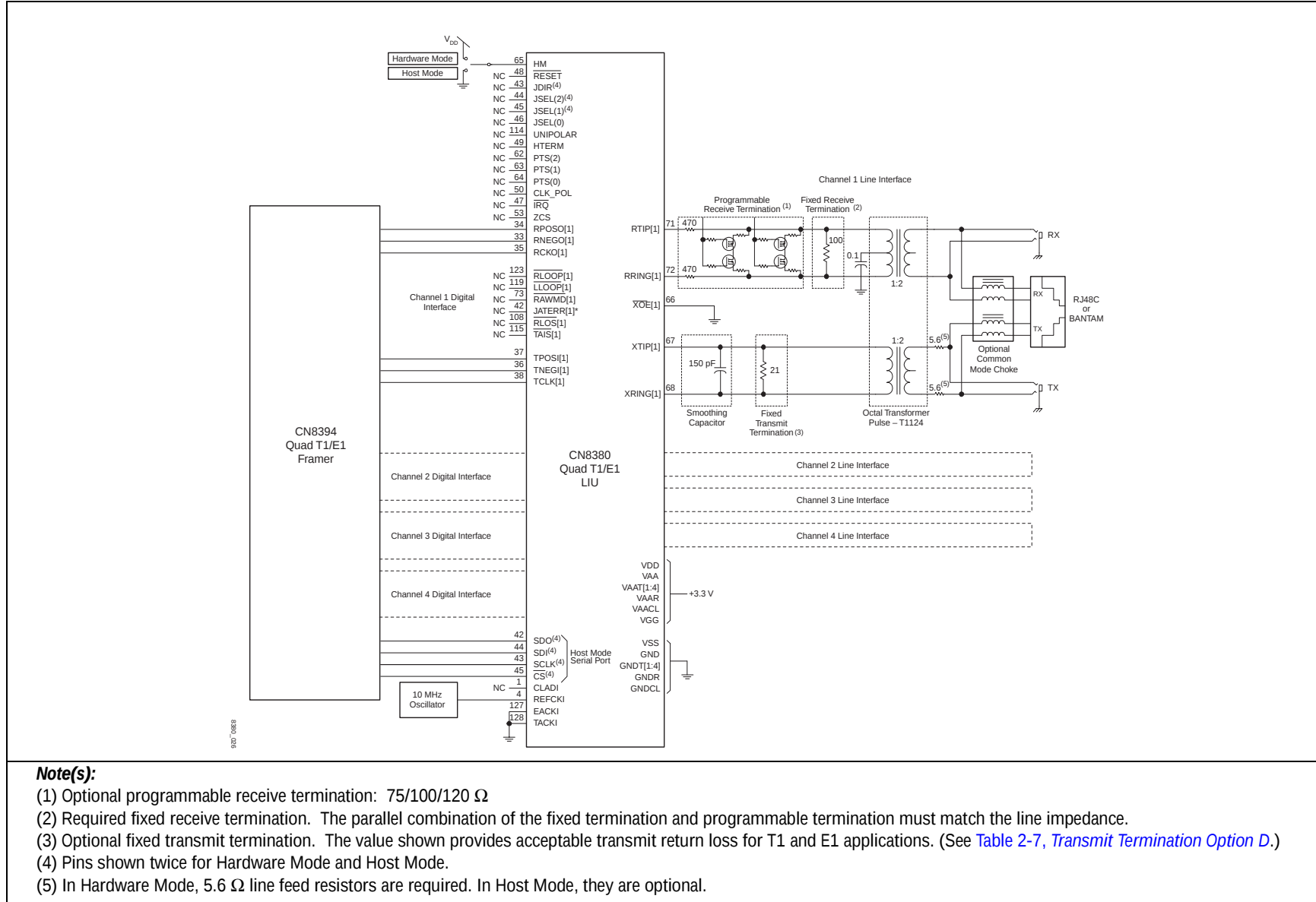
Figure B-1. Minimum Hardware Configuration
