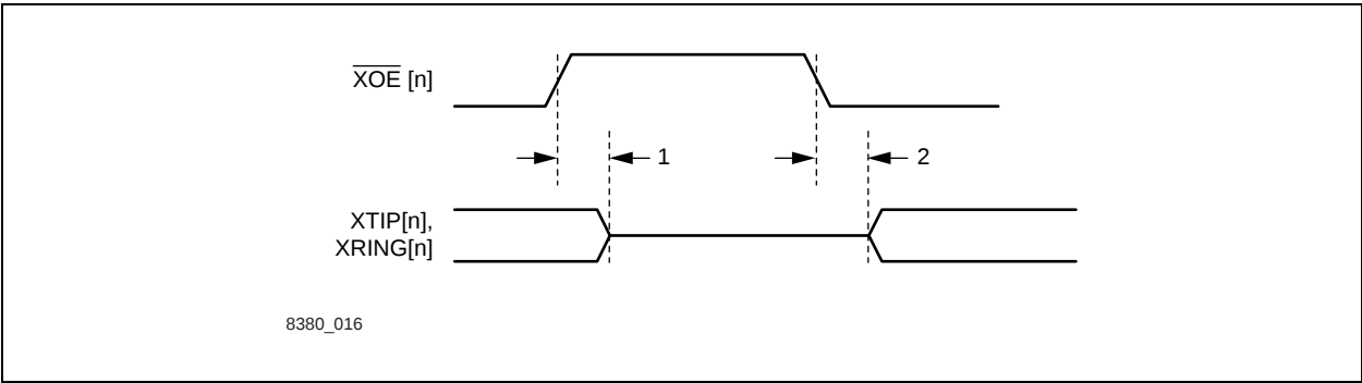
Figure 4-1. \overline{\text{XOE}} Timing Diagram
