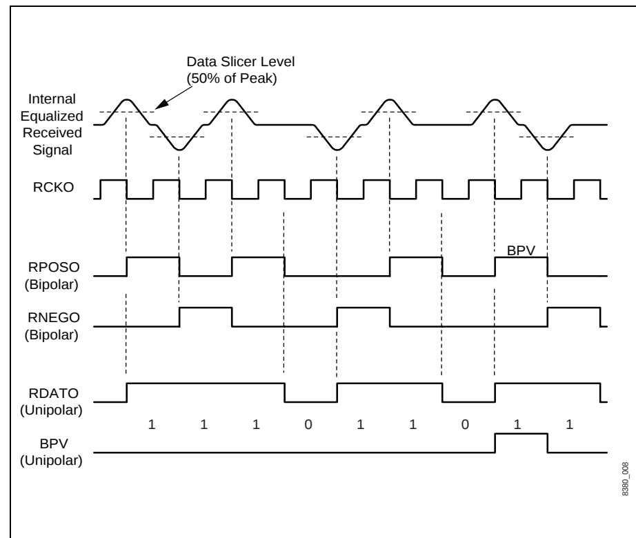
Figure 2-3. Receiver Signals
