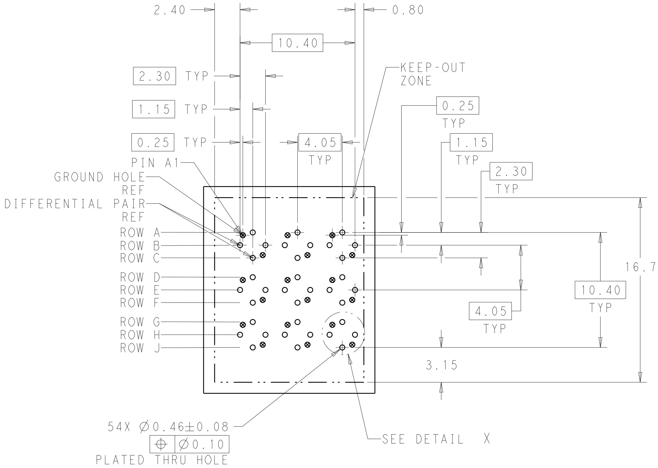
UNGUIDED BACKPLANE HOLE PATTERN (CONNECTOR SIDE)
