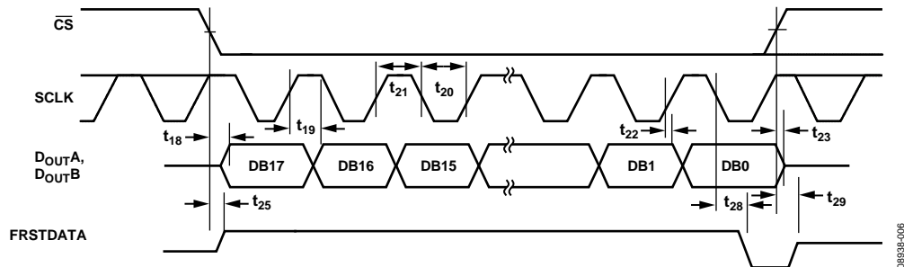
Figure 6. Serial Read Operation (Channel 1)
