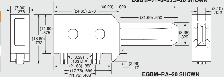
EGBM-RA-20 SHOWN
