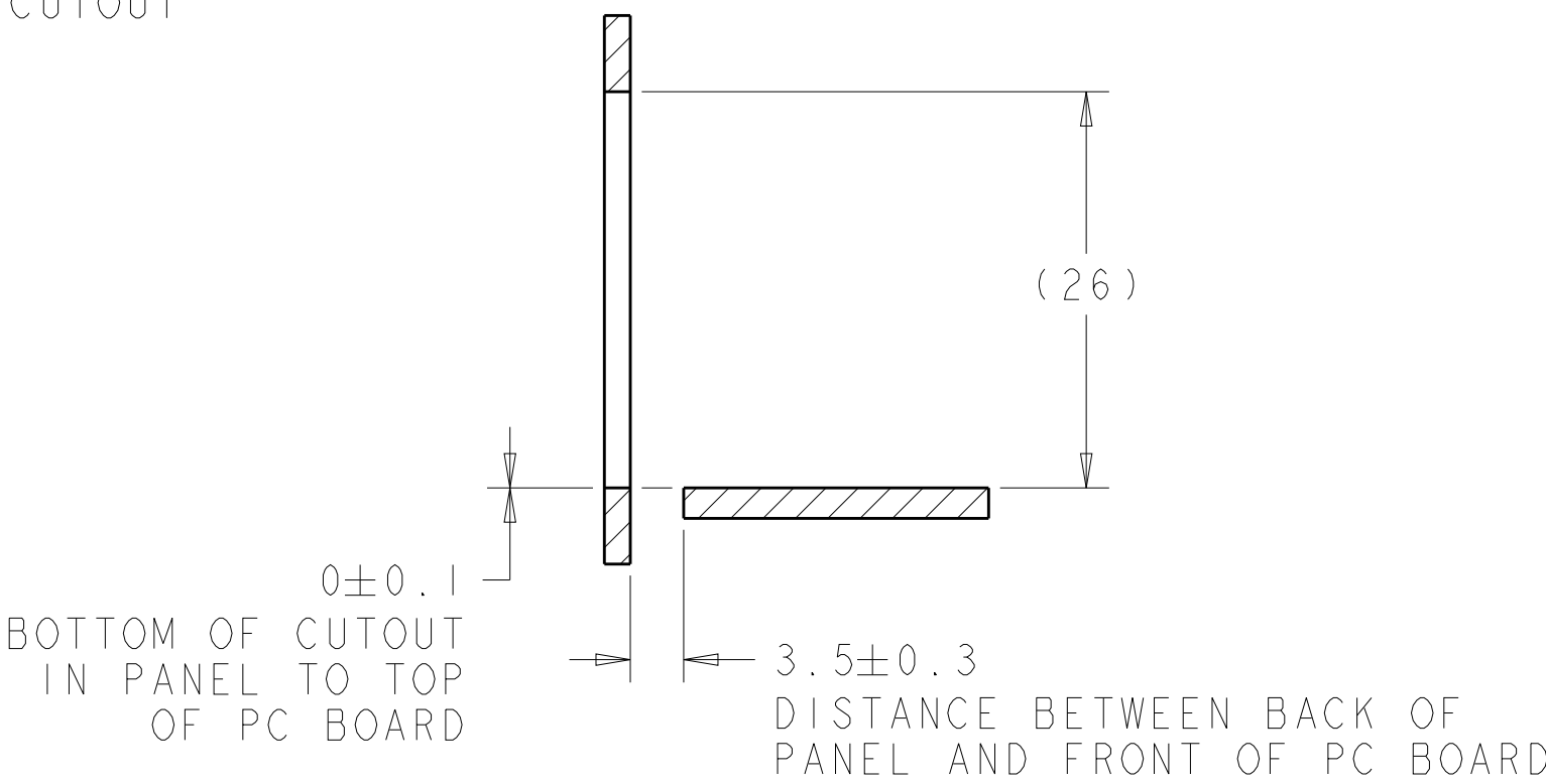
SECTION U-U
