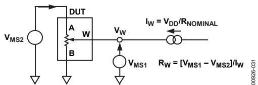
Figure 24. Wiper Resistance
