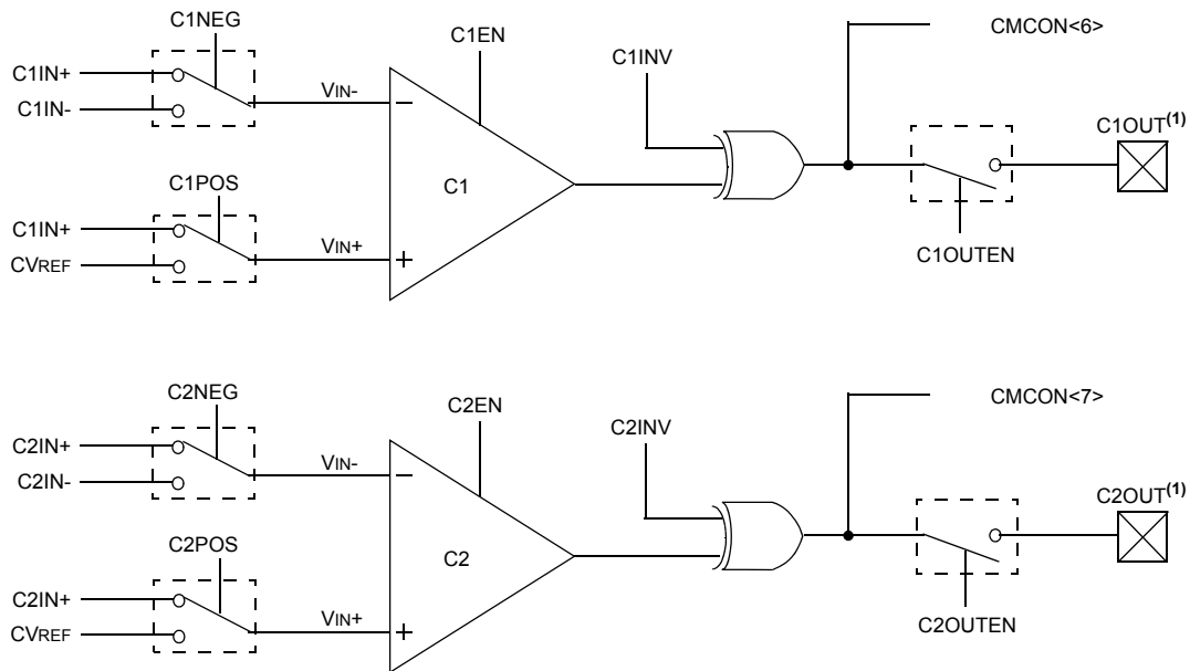
FIGURE 21-1: COMPARATOR I/O OPERATING MODES
