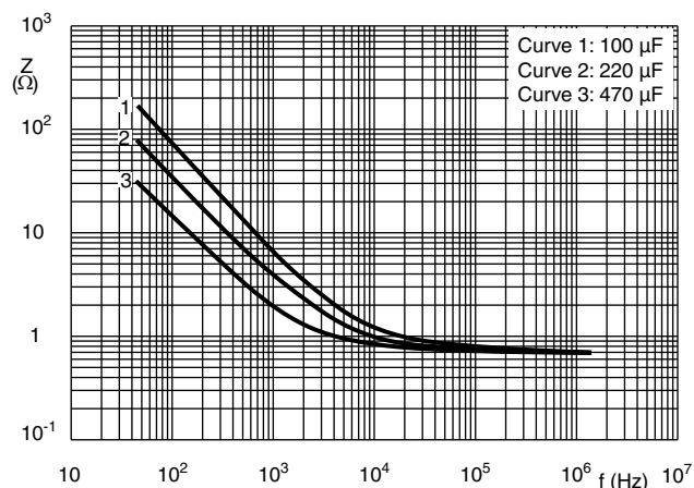
Fig. 12 - Typical impedance as a function of frequency T_{\text{amb}} (^\circ\text{C})
