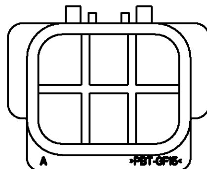
4 POS 2040594-3 SCALE 2:1
