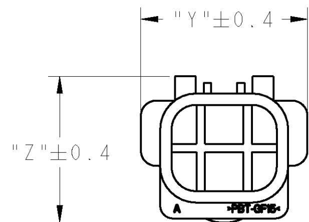
2 POS 2040594-1 SCALE 2:1
