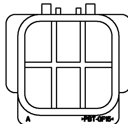
6 POS 2040594-4 SCALE 2:1
