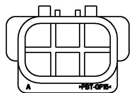
3 POS 2040594-2 SCALE 2:1
