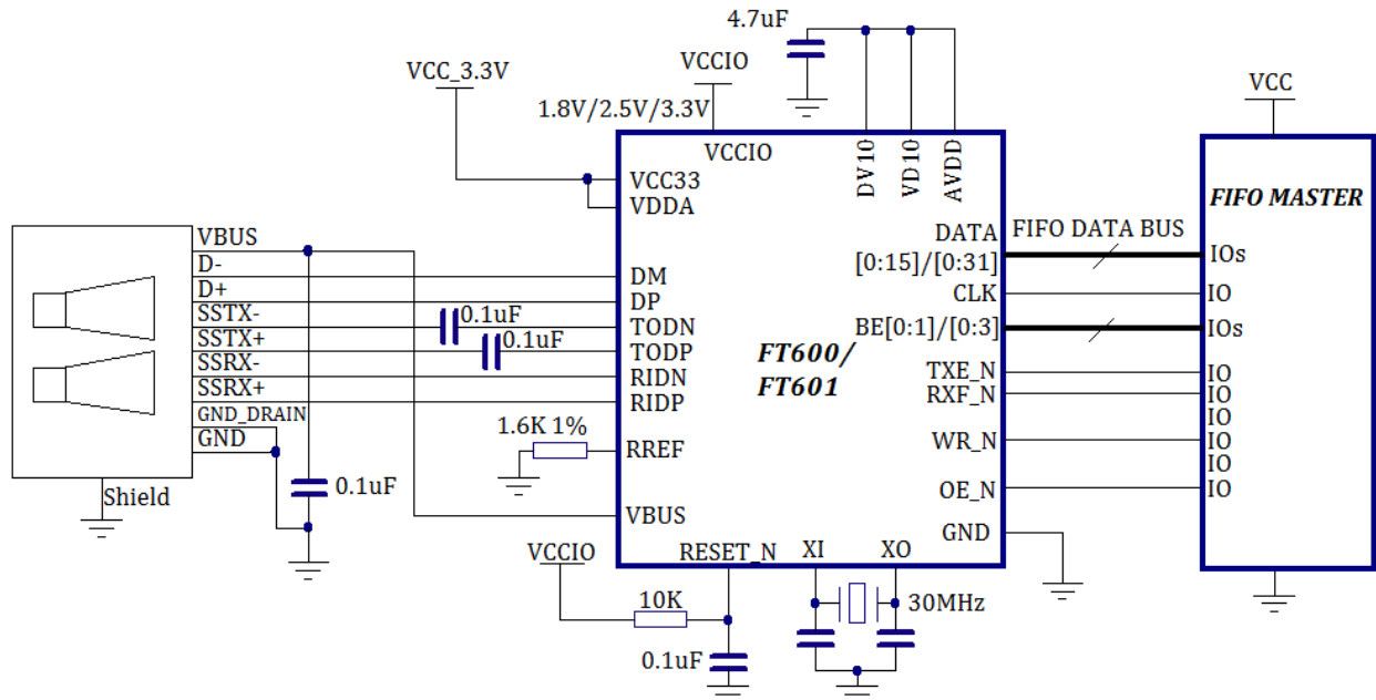
Figure 7.1 FT600/FT601 Connect to FIFO Master Interface (Multi-Channel FIFO Mode)
