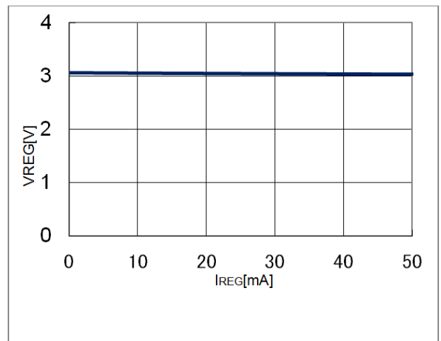
Figure 11. V REG output voltage vs REG load current
