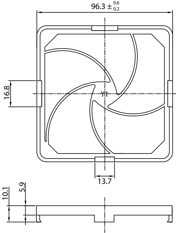
RETAINER
