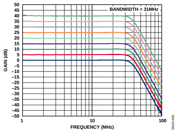
Figure 6. Gain vs. Frequency over V_{\text{GAIN}} (Bandwidth Setting = 31 MHz)
