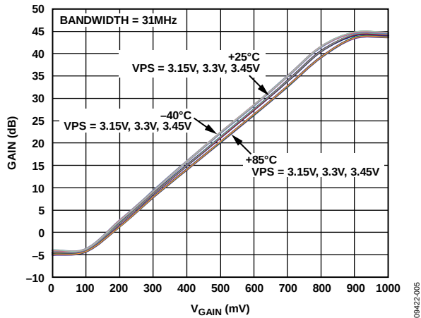
Figure 5. In-Band Gain vs. V_{\text{GAIN}} over Supply and Temperature (Bandwidth Setting = 31 MHz)
