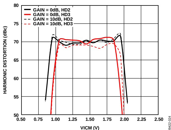
Figure 23. HD2 and HD3 vs. Input Common-Mode Voltage (Bandwidth Setting = 31 MHz, 0.4 V p-p Input Level)
