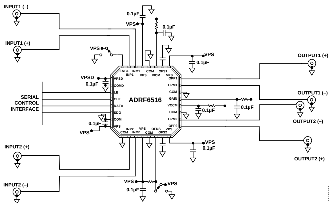
Figure 51. Basic Connections
