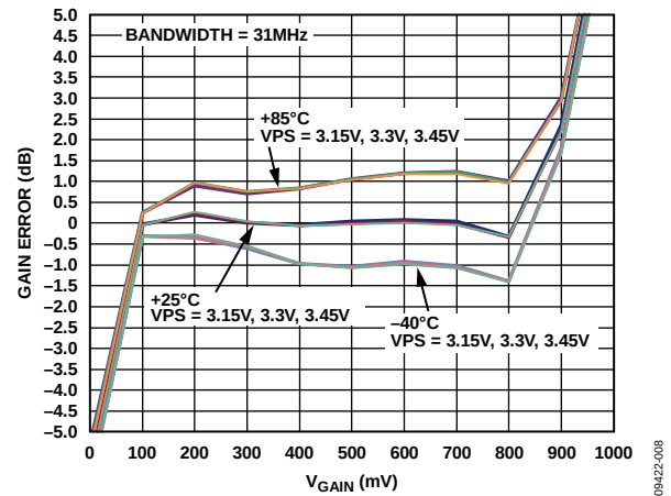
Figure 8. Gain Conformance vs. V_{\text{GAIN}} over Supply and Temperature (Bandwidth Setting = 31 MHz)
