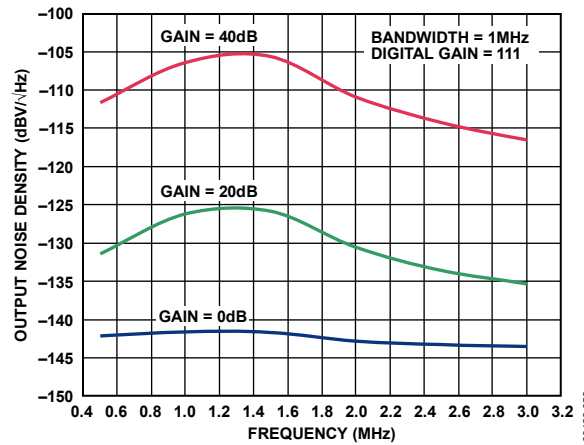
Figure 34. Output Noise Density vs. Frequency (Bandwidth Setting = 1 MHz, Digital Gain = 111)
