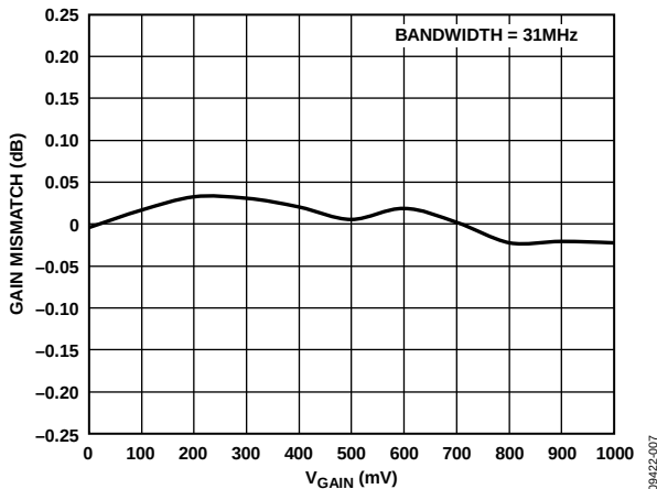
Figure 7. Gain Matching vs. V_{\text{GAIN}} (Bandwidth Setting = 31 MHz)
