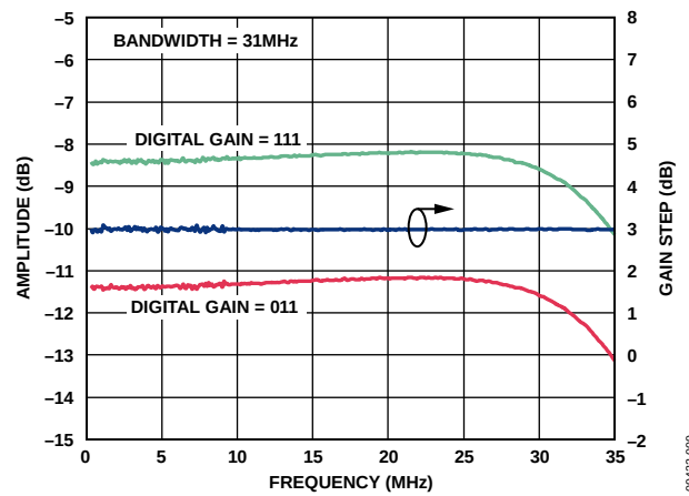
Figure 9. Gain Step and Gain Error vs. Frequency (Bandwidth Setting = 31 MHz, V_{\text{GAIN}} = 0\text{ V} )
