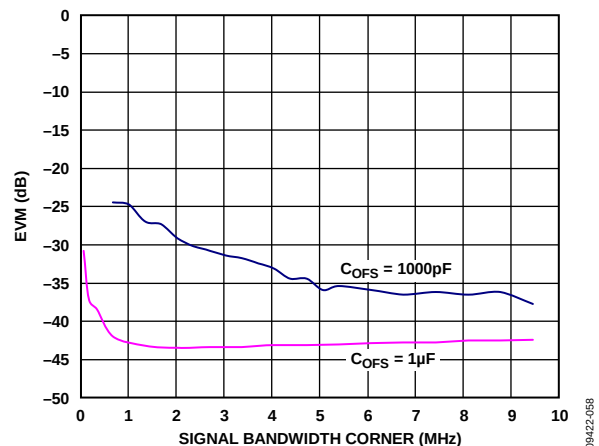
Figure 56. EVM vs. Signal Bandwidth Corner with C_{OFS} = 1 \mu\text{F} and C_{OFS} = 1000 \text{ pF} (Filter Corner = 10 MHz)
