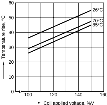
2.-(2) Coil temperature rise Sample: 5 pcs., JS1a-24V-F Measured portion: Inside the coil Contact current: 10 A
