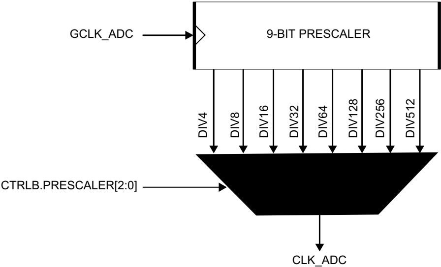
Figure 29-2. ADC Prescaler
