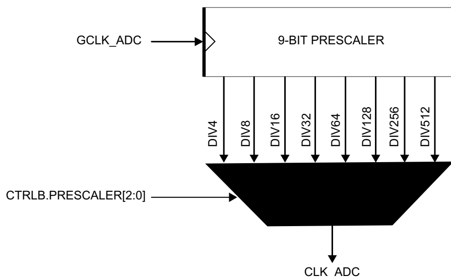
Figure 29-2. ADC Prescaler
