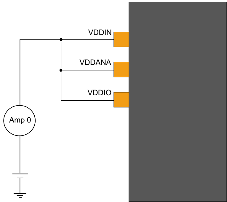
Figure 30-1. Measurement Schematic
