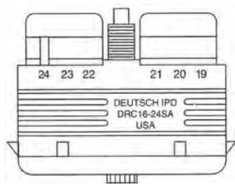
Standard Plug
