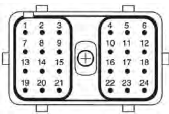
In-line Receptacle
