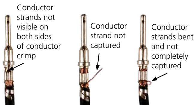
Unacceptable Crimps
