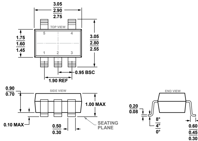
COMPLIANT TO JEDEC STANDARDS MO-193-AB Figure 69. 5-Lead Thin Small Outline Transistor Package [TSOT] (UJ-5) Dimensions shown in millimeters
