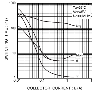
Fig.13 Switching time
