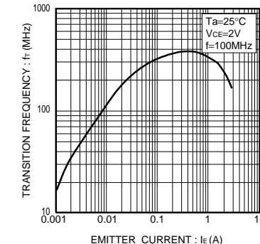
Fig.12 Gain bandwidth product vs. emitter current
