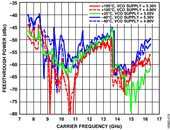
Figure 19. RF16P and RF16N VCO x 3 Feedthrough, De-Embedded Board and Cable Measurement, Combined Using Balun
