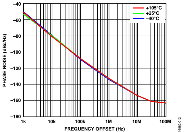
Figure 12. Open-Loop VCO Phase Noise over Temperature, 8.0 GHz, VCC_VCO = 5 V
