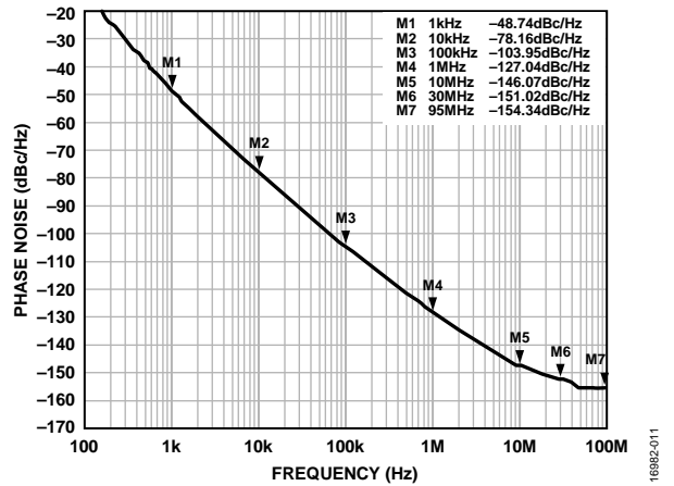
Figure 11. Open-Loop VCO Phase Noise at RF16x Output, 16.0 GHz, VCC_VCO = 5 V
