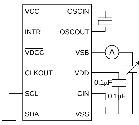
Test Circuit
