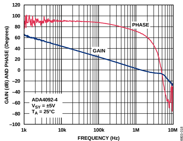
Figure 18. Open-Loop Gain and Phase vs. Frequency, 10 V
