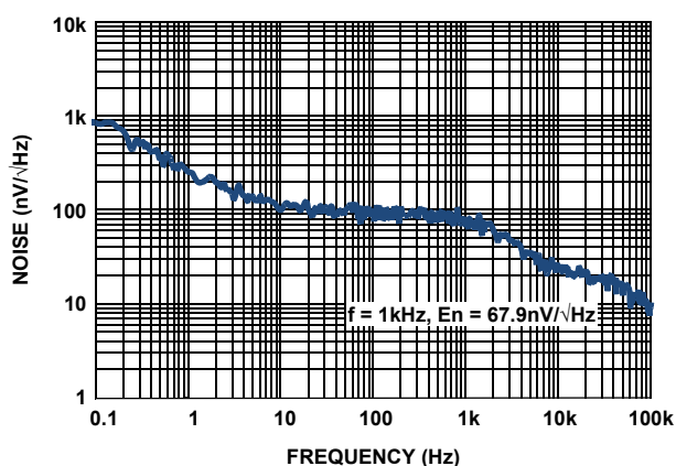
FIGURE 11. NOISE DENSITY vs FREQUENCY ( V_{IN} = 7.1V , I_{OUT} = 0mA , C_{IN} = 0.1\mu F , C_{OUT} = 1\mu F , COMP = 1nF )
