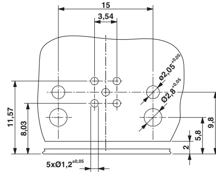
Drilling diagram only valid in connection with the SACC-M12-SCO NUT L90 housing (order no. 1432460)
