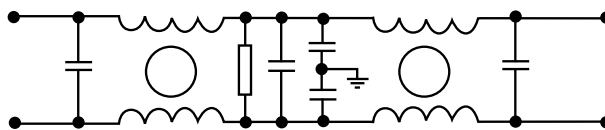
Circuit 2
