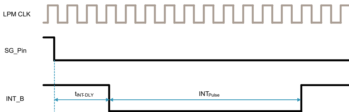
Figure 6. Interrupt pulse timer
