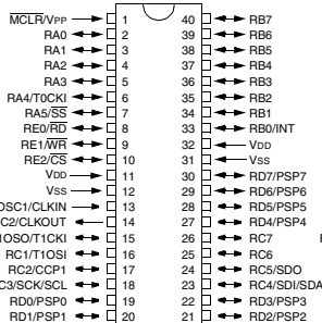
PIC16C64A PIC16CR64
