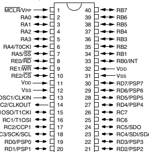
PIC16C64A PIC16CR64
