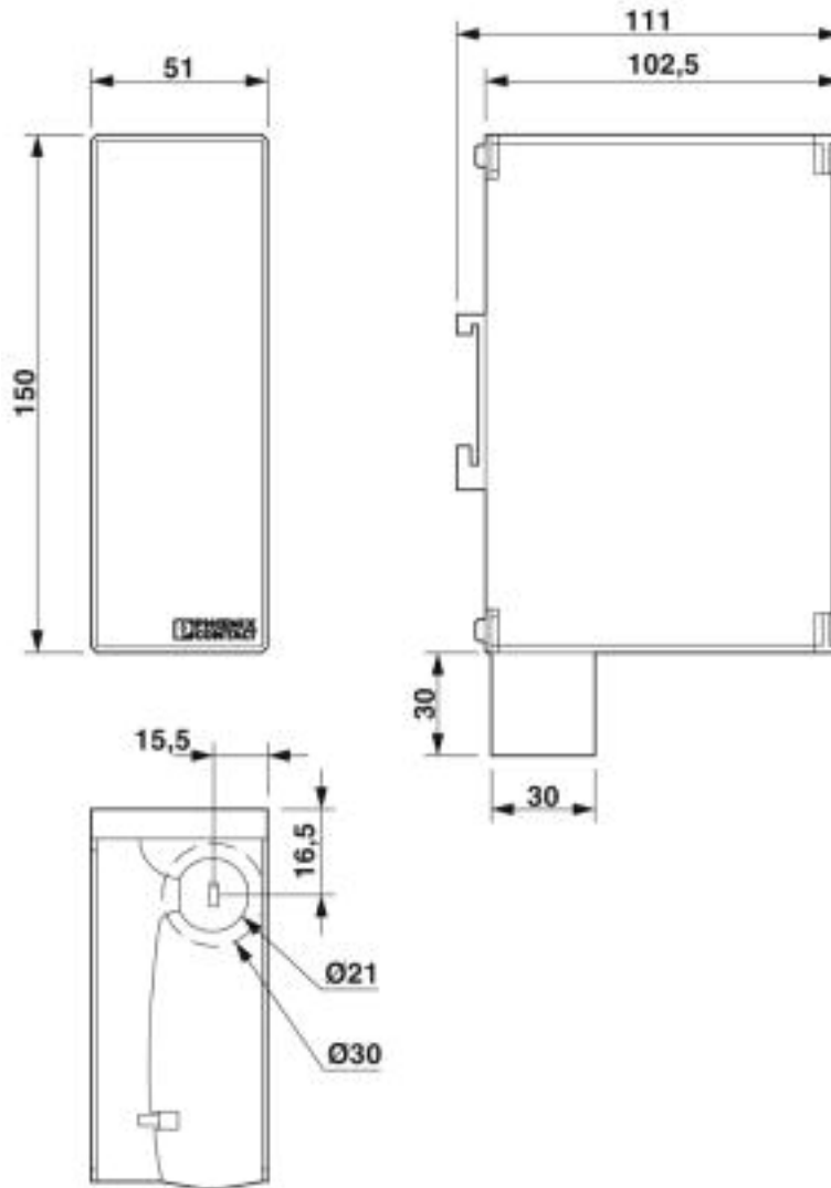
Dimensional drawing
