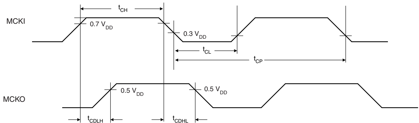
Figure 3. Clock Waveform
