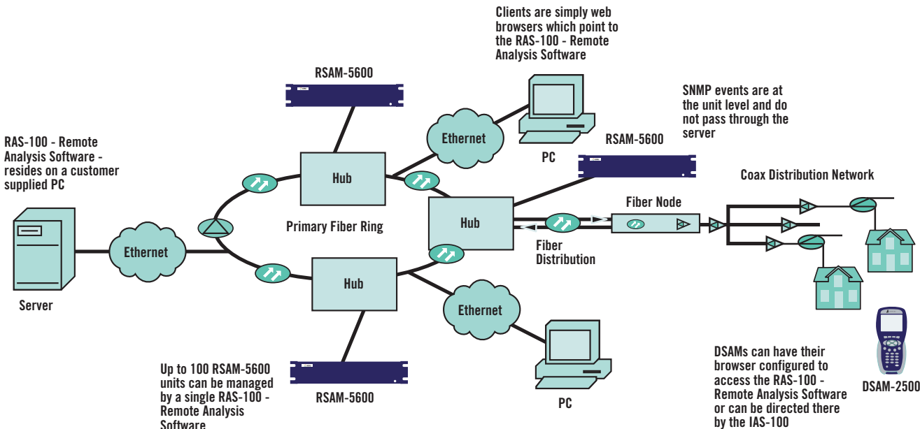
Figure 1: Typical instalation
