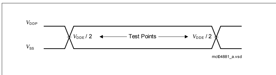
Figure 11 Testing Waveform, Output Delay
