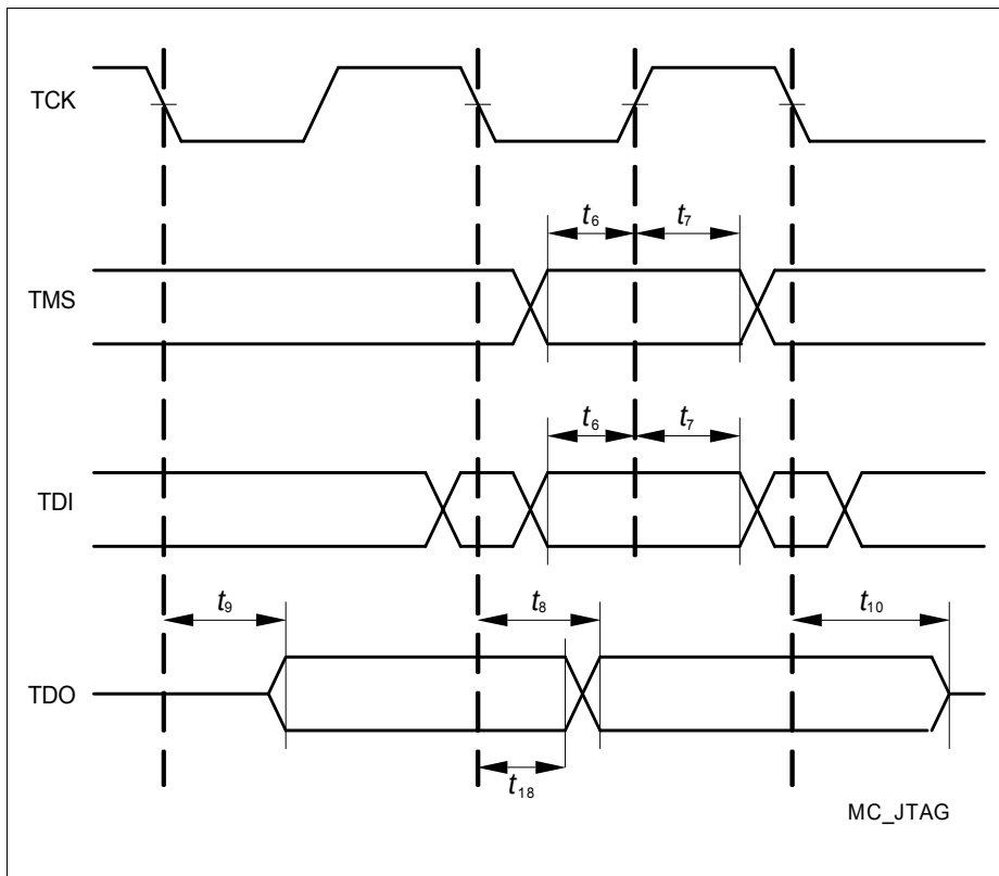
Figure 18 JTAG Timing
