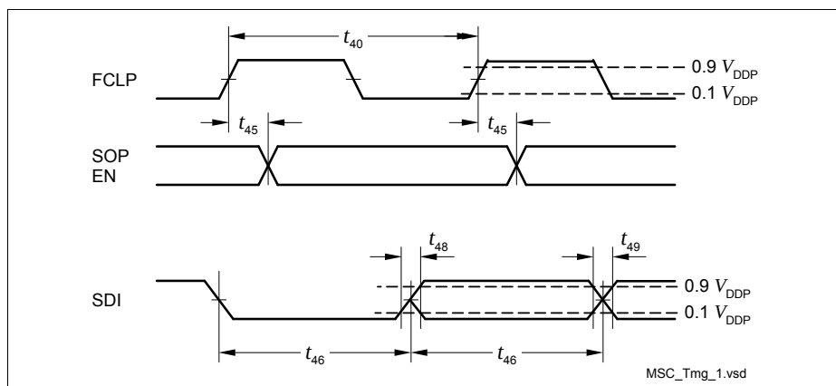
Figure 23 MSC Interface Timing
