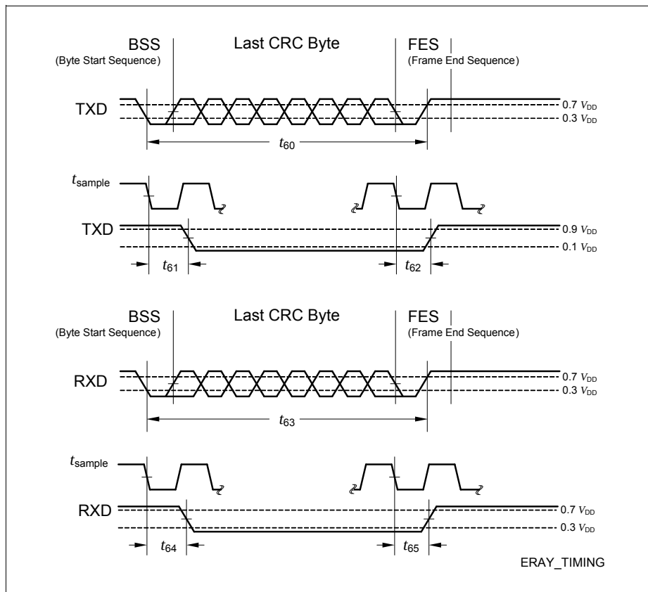
Figure 26 ERAY Timing
