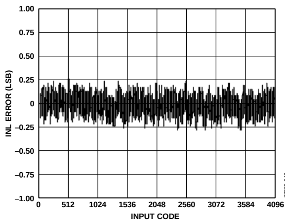
Figure 14. Typical AD5391-5 INL Plot
