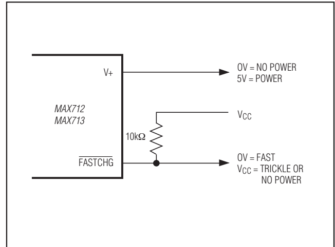
Figure 17. Logic-Level Status Outputs
