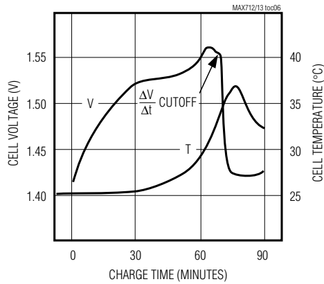
MAX713 NiCd BATTERY-CHARGING CHARACTERISTICS AT C/2 RATE
