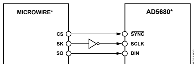
Figure 30. AD5680 to MICROWIRE Interface
