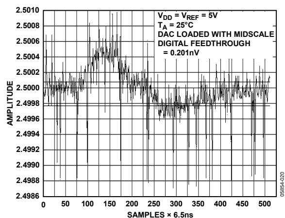
Figure 17. Digital Feedthrough
