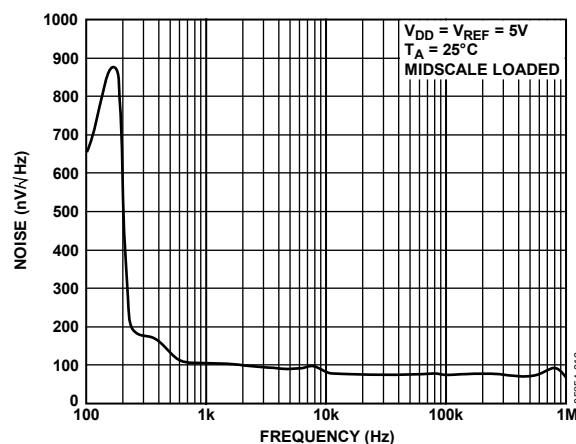
Figure 21. Noise Spectral Density
