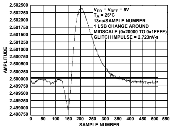
Figure 16. Digital-to-Analog Glitch Impulse (Negative)
