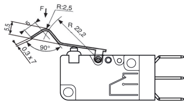
161F dummy roller
