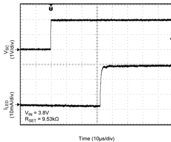
ILED Response to SC Signal Turn-On Time
